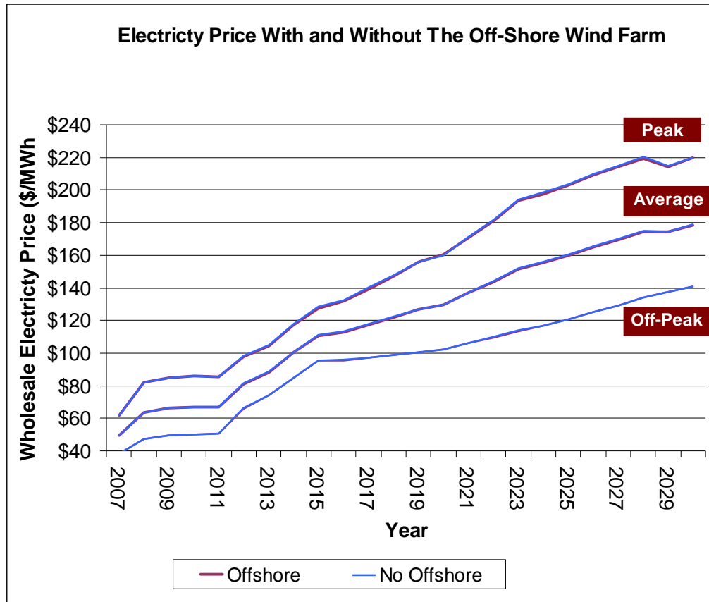
Figure 3.3: Electricity Price With and Without Wind
